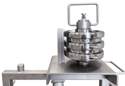
Knife cassette of scanEmul 175 - Hopper fed shown assembled.
