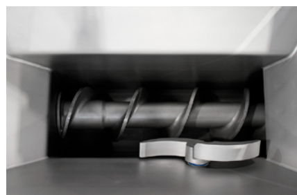
SuperPump SP 290 infeed hopper shown with rotating feeding device for feeding screw.
