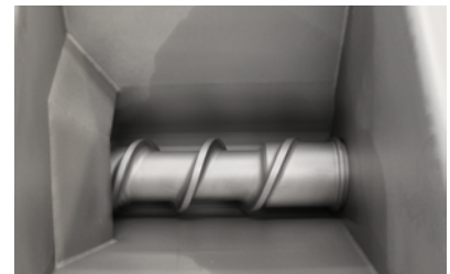
View of hopper infeed of MC 300 - Hopper fed
