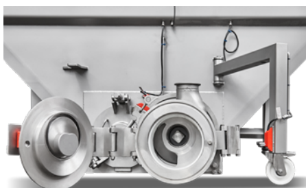
ContiPump pump housing, hinged.
