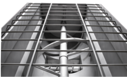
2500 L silo/buffer hopper with stirring/feeding device. The stirring device feeds product to the centre for discharge into SuperPump SP 200.
