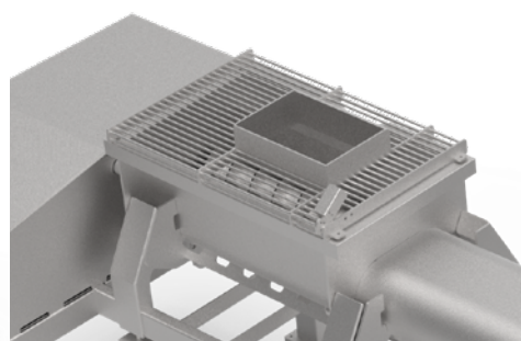
View of hopper infeed of MC 300 - Screw hopper fed
